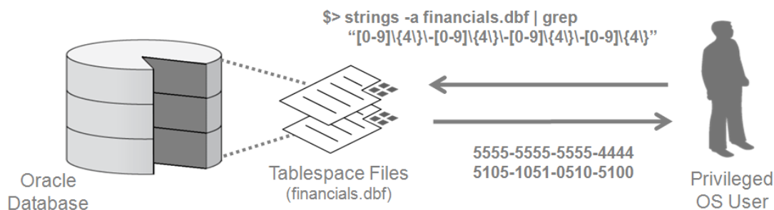
Figure 1. Extracting customer credit card numbers from Oracle database tablespace files
