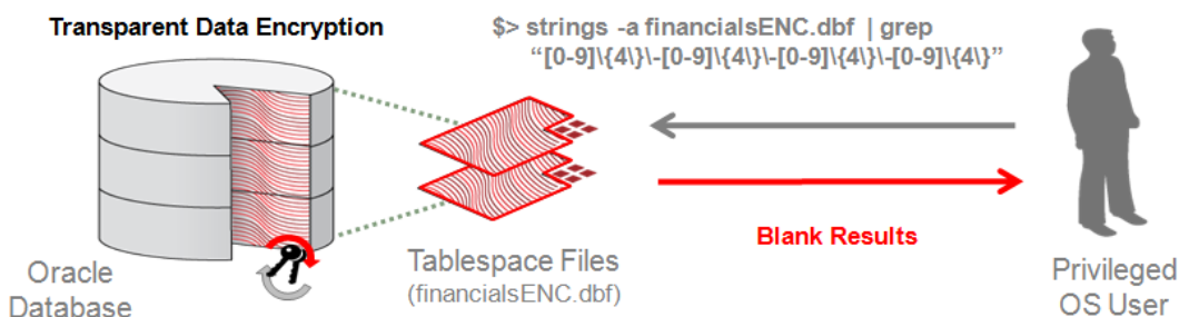
Figure 2. Encrypting with Transparent Data Encryption to prevent database bypass
