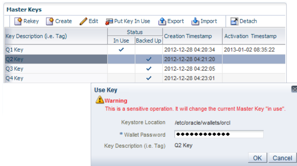
Figure 4. Managing and rotating TDE master keys using Oracle Enterprise Manager
