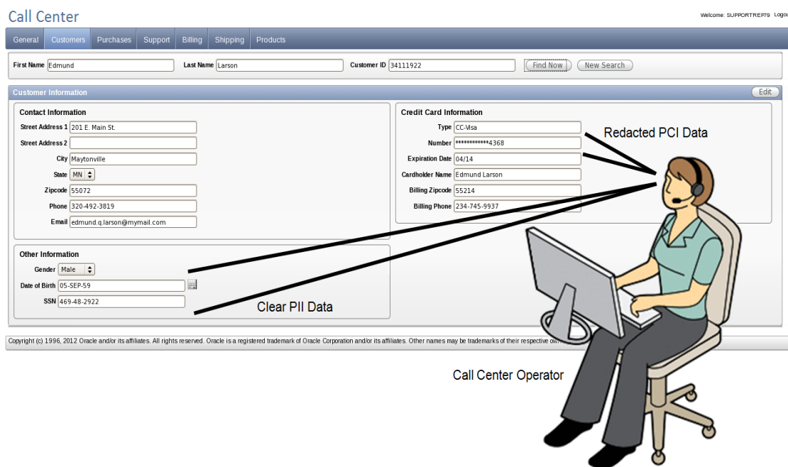
Figure 6. Clear and redacted information displayed in a call center application
