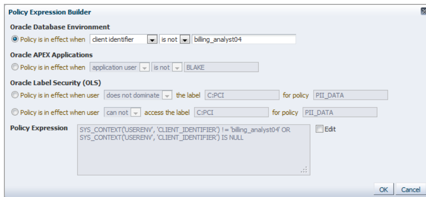
Figure 9. Using Oracle Enterprise Manager Policy Expression Builder to create Data Redaction policies
